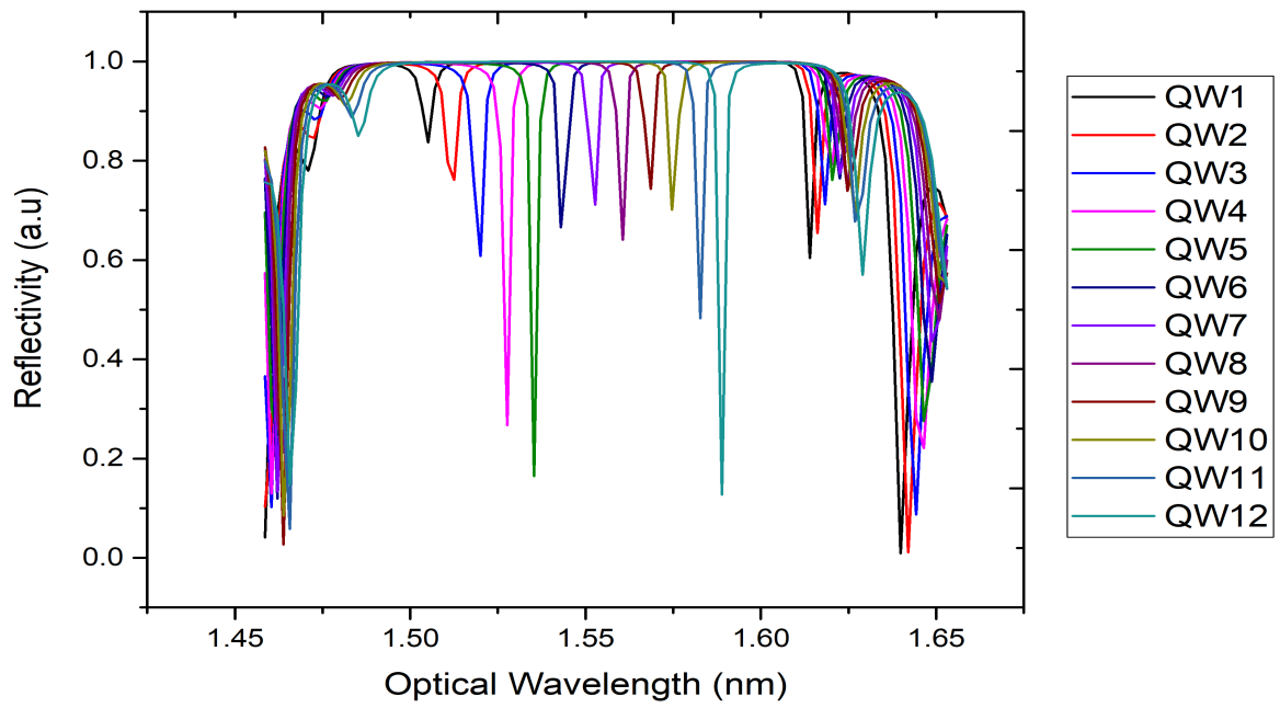
FIGURE 4.15: Reflectivity vs optical wavelength for 30:28 mirror ratio.
