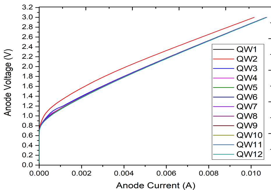
FIGURE 4.24: Anode voltage vs anode current for 45:43 mirror ratio.
