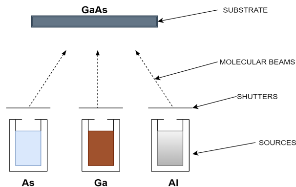
FIGURE 2.26: Vaporisation cells inside a high-vacuum chamber cylindrical beakers of Al, Ga, As liquid do-pants onto a GaAs layer.
