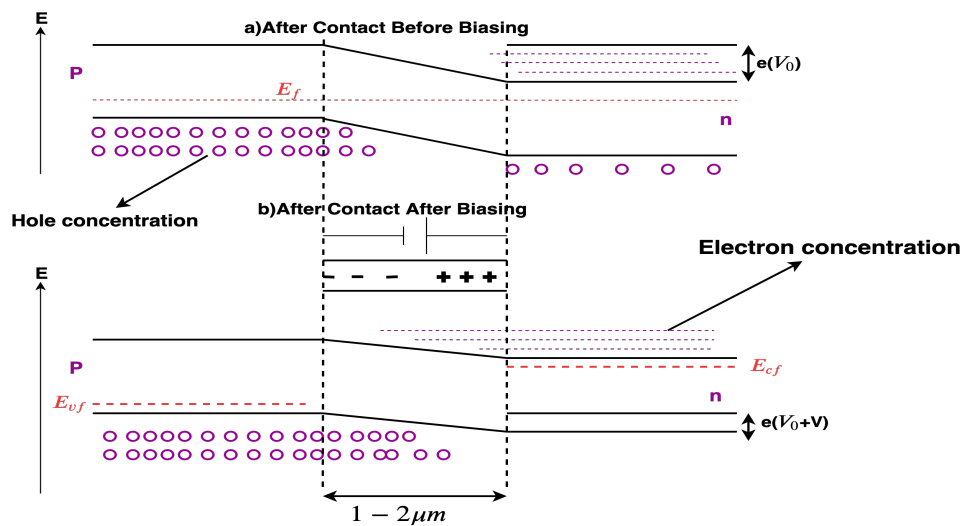
FIGURE 2.21: Homo junction after contact, before and after biasing.
