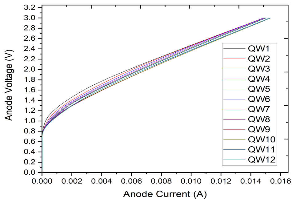
FIGURE 4.23: Anode voltage vs anode current for 30:28 mirror ratio.
