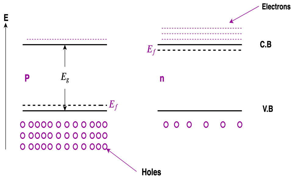
FIGURE 2.20: Homo junction before contact.
