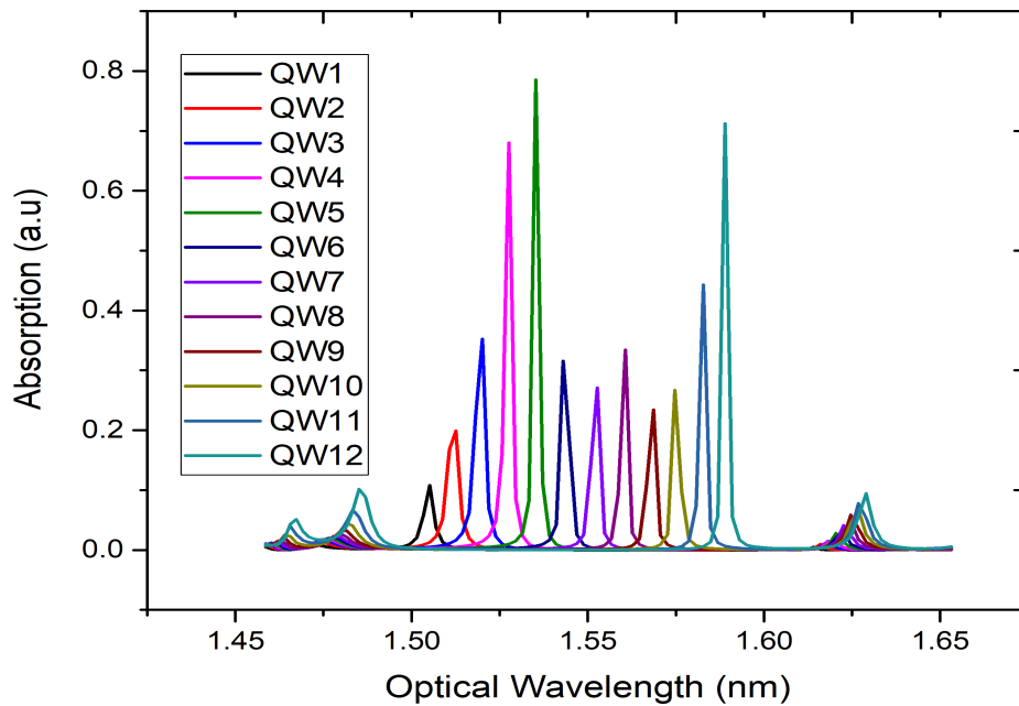
FIGURE 4.13: Absorption vs optical wavelength for 30:28 mirror ratio.
