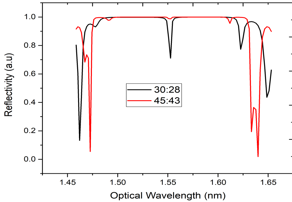
FIGURE 4.7: Reflectivity for 30:28 and 45:43 structures.
