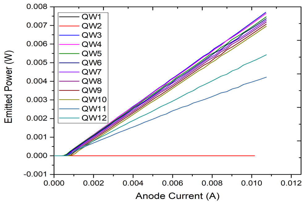
FIGURE 4.20: Emitted power vs anode current for 45:43 mirror ratio.
