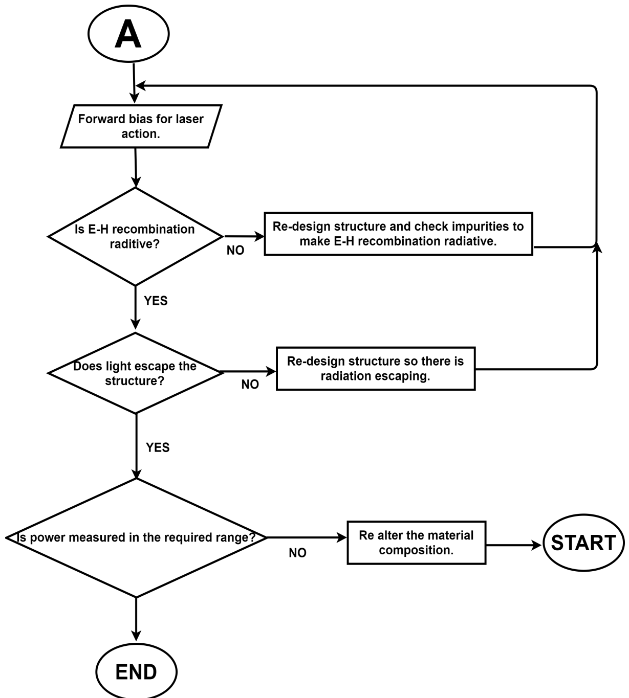
FIGURE 3.3: VCSEL development flowchart continuation.
