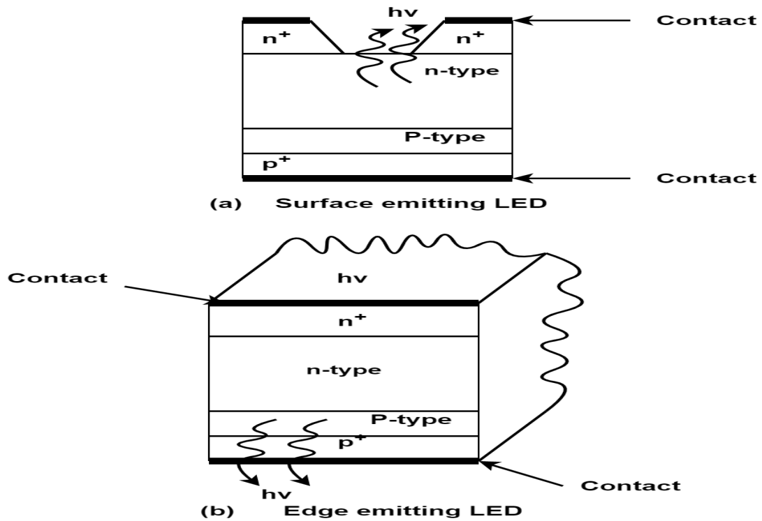
FIGURE 2.8: Types of LEDs
