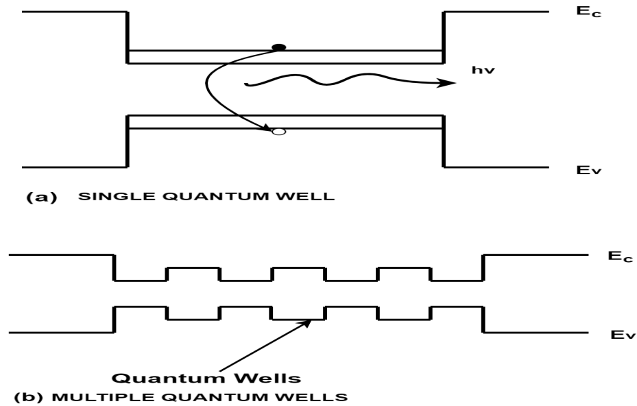
FIGURE 2.18: Quantum Well laser structures (a) showing a single quantum (b) Multiple Quantum Wells.
