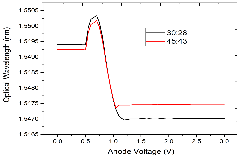
FIGURE 4.4: Optical wavelength vs anode voltage for 30:28 and 45:43 vcsel structures.
