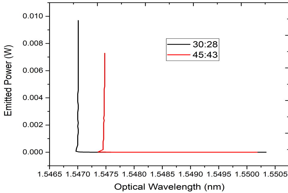
FIGURE 4.5: Emitted power against optical wavelength for 30:28 and 45:43 structures.
