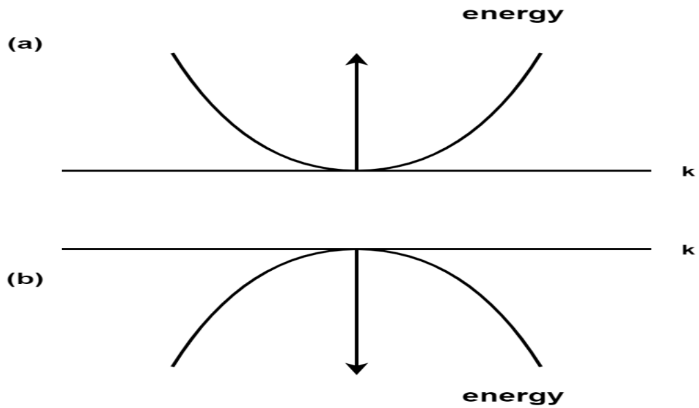
FIGURE 2.6: energy v.s k relationship for (a) conduction band and (b) valence band with parabolic curves and E(k) centred about = 0
