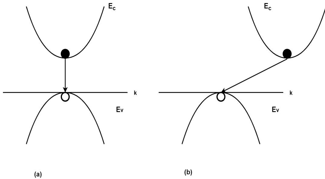
FIGURE 2.7: (a) direct band gap semiconductor showing electron-hole recombination sketch. (b) indirect band gap electron-hole semiconductor sketch.
