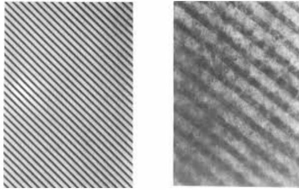
FIGURE 2.27: Cross section of MBE-grown crystal with layers of GaAs(dark) and AlGaAs (light) [3].
