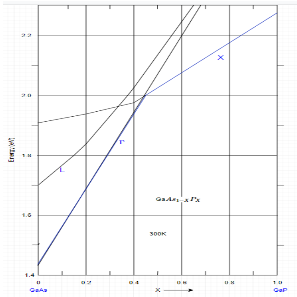
FIGURE 2.23: Conduction band energies of GaAsP.
