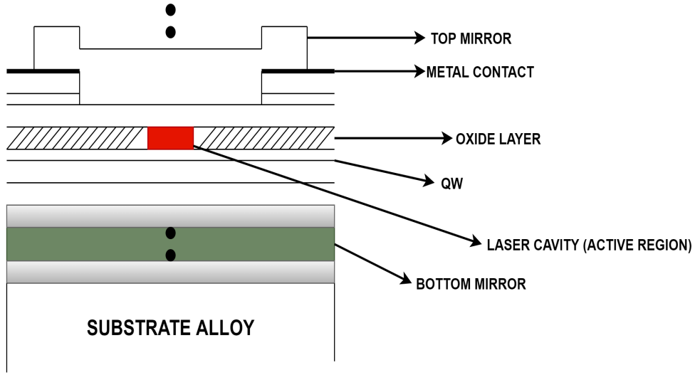
FIGURE 2.24: Typical VCSEL structure.
