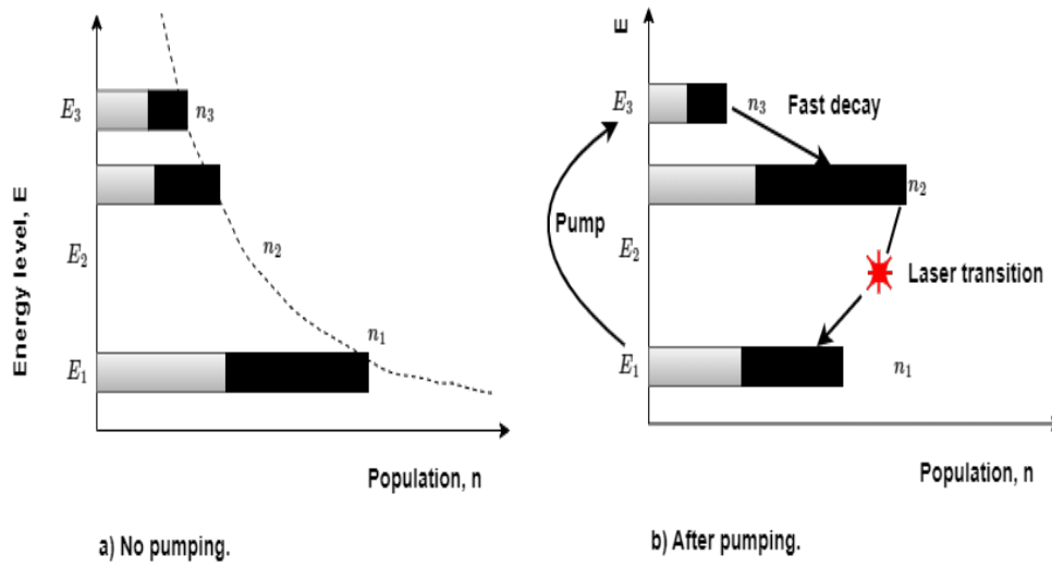
FIGURE 2.15: Three level system.
