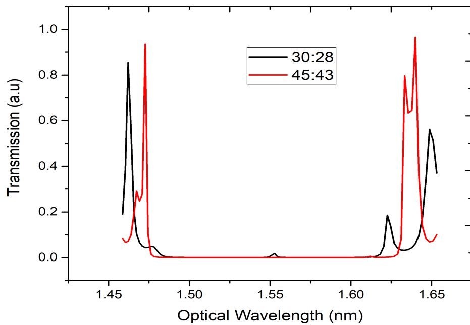
FIGURE 4.8: Wavelength transmission for 30:28 and 45:43 structures.
