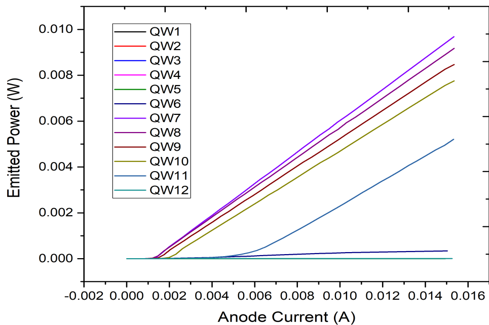
FIGURE 4.19: Emitted power vs anode current for 30:28 mirror ratio.
