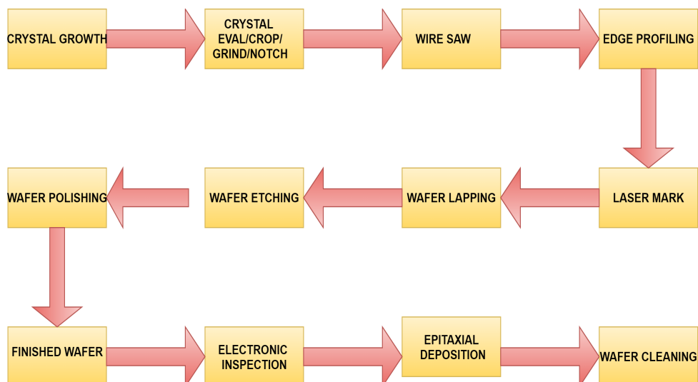
FIGURE 2.25: Steps involved in manufacturing Si wafers.
