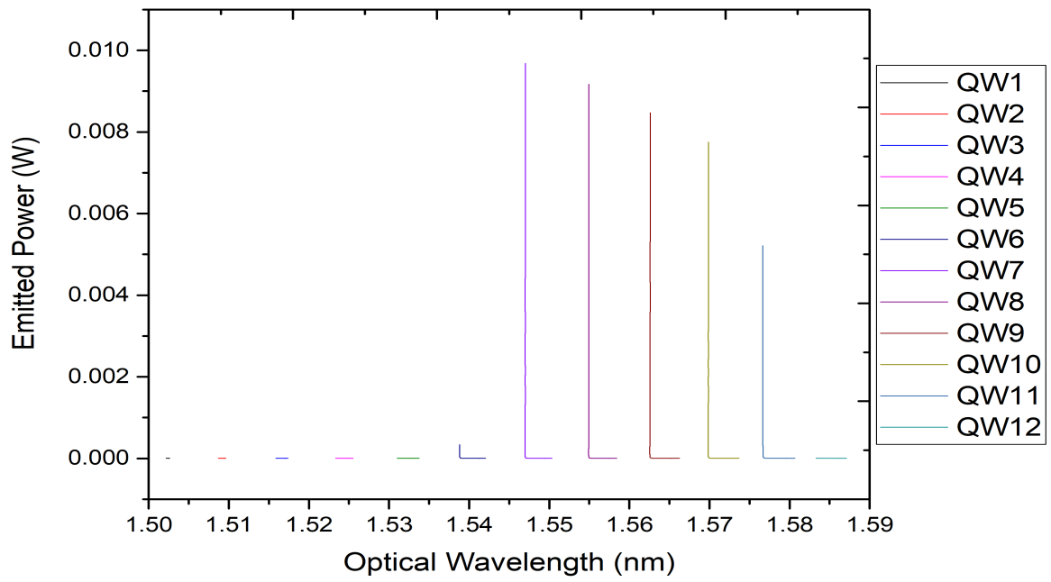
FIGURE 4.11: Emitted power vs optical wavelength for 30:28 mirror ratio.
