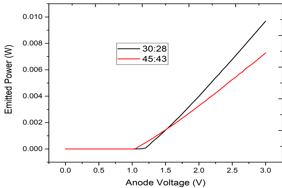
FIGURE 4.2: Emitted power vs Anode voltage.
