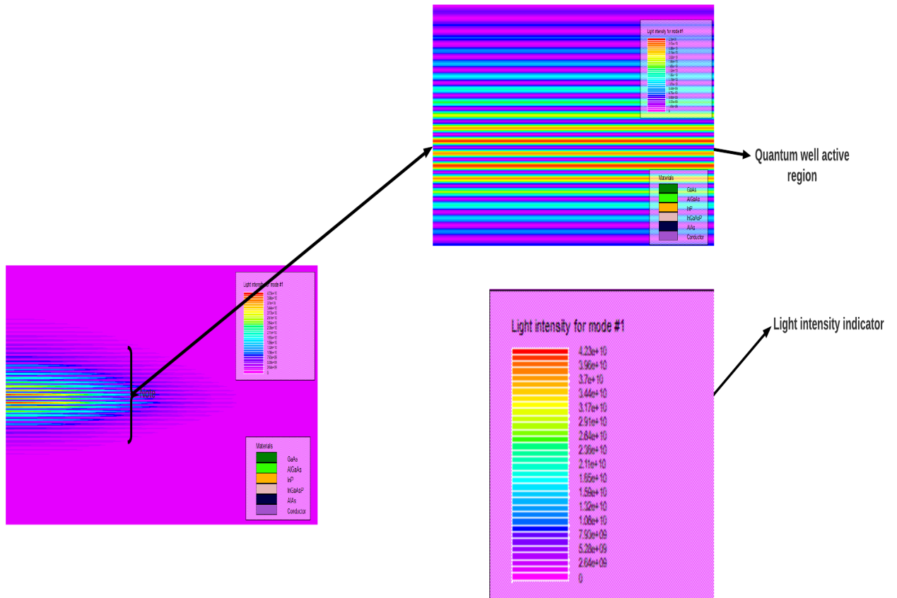
FIGURE 3.6: Figure showing light intensity distribution in the Vcsel structure.
