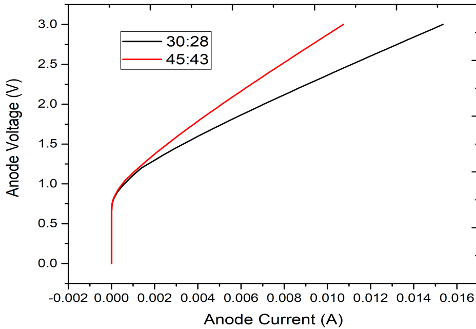
FIGURE 4.3: Anode voltage vs Anode current.
