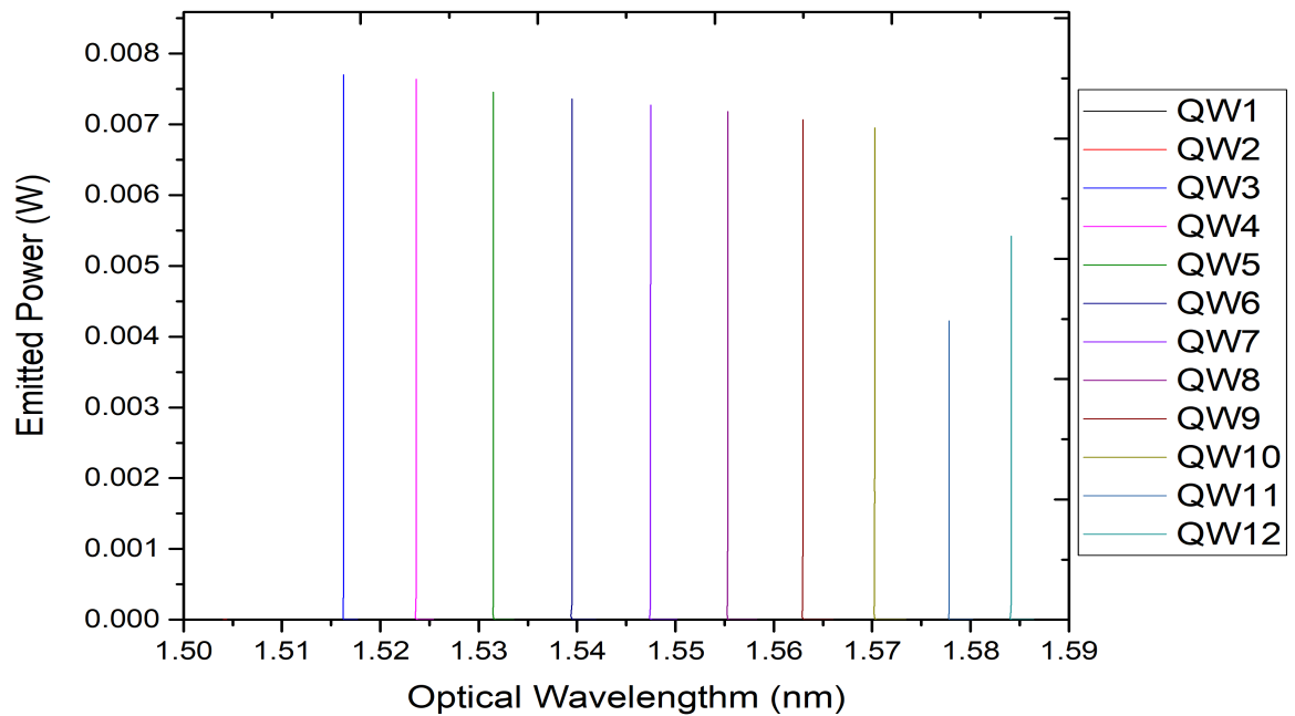
FIGURE 4.12: Emitted power vs optical wavelength for 45:43 mirror ratio.
