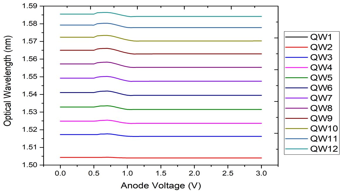
FIGURE 4.10: Optical wavelength vs anode voltage for 45:43 mirror ratio.
