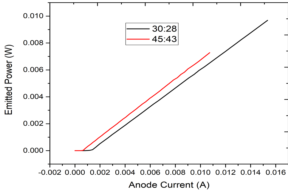
FIGURE 4.1: Emitted power vs Anode Current.
