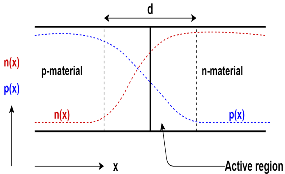
FIGURE 2.19: Carrier distribution across a homo junction.
