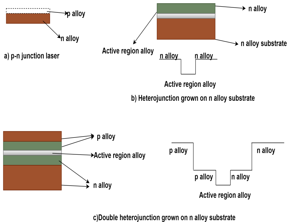
FIGURE 2.17: Junction laser structures.
