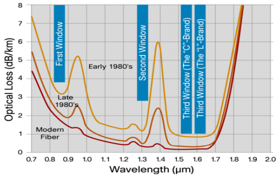
FIGURE 2.2: Attenuation V.S wavelength for a fused silica optical fibre [2].
