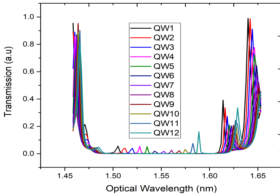
FIGURE 4.17: Transmission vs optical wavelength for 30:28 mirror ratio.
