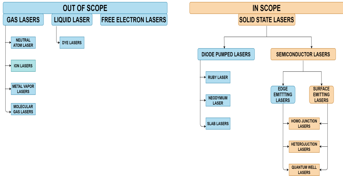
FIGURE 2.9: Classifications of lasers.
