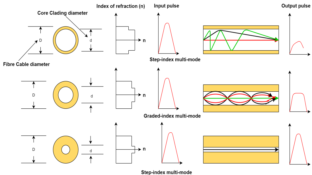
FIGURE 2.5: Fibre types [2].
