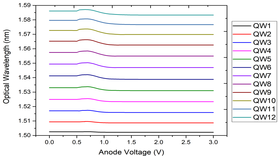
FIGURE 4.9: Optical wavelength vs anode voltage for 30:28 mirror ratio.
