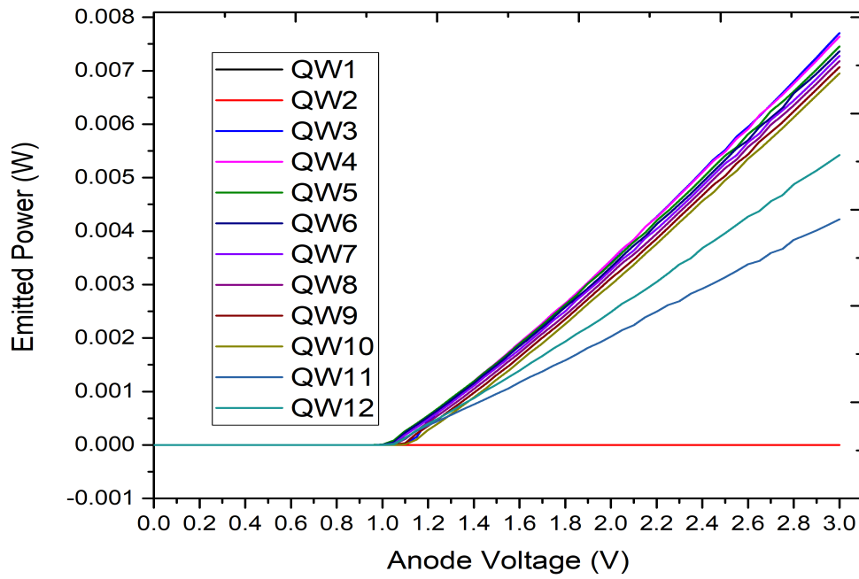
FIGURE 4.22: Emitted power vs anode voltage for 45:43 mirror ratio.
