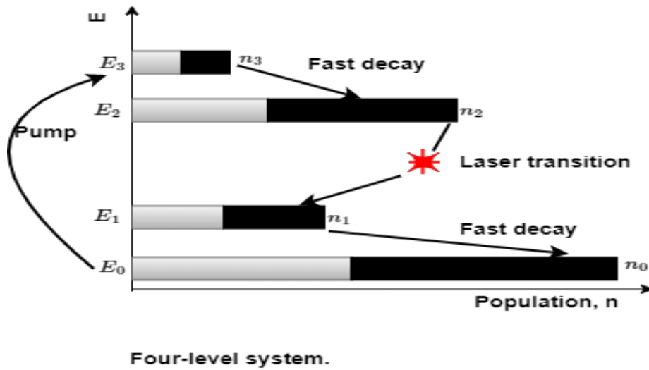
FIGURE 2.16: Four level system.
