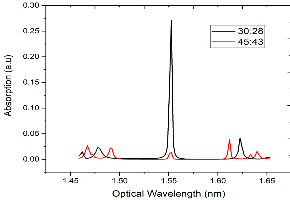
FIGURE 4.6: Absorption for 30:28 and 45:43 vcsel structure.
