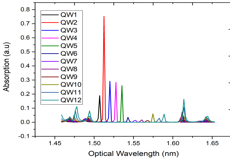
FIGURE 4.14: Absorption vs optical wavelength for 45:43 mirror ratio.
