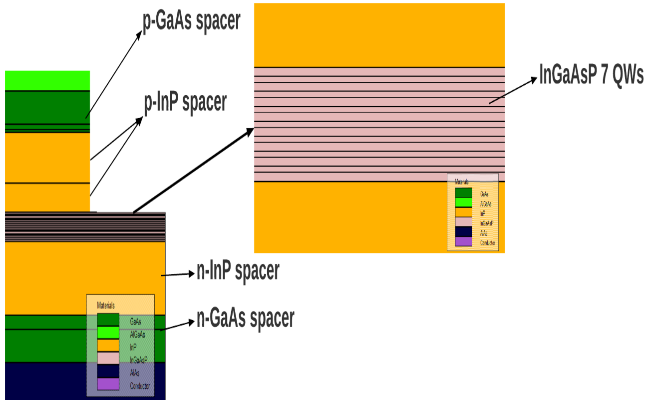
FIGURE 3.5: P-doped and n-doped regions sandwiching an InGaAsP seven quantum well active region.
