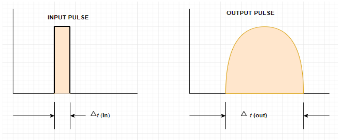
FIGURE 2.3: Pulse Spreading Caused by Dispersion.
