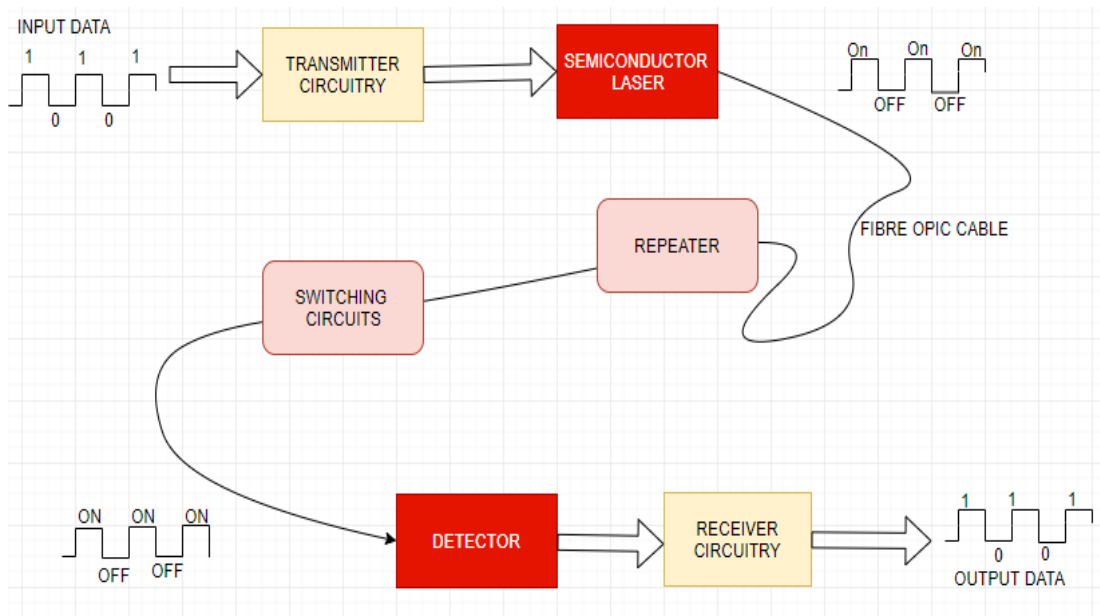
FIGURE 2.4: Schematic of a fibre communication system showing amplifiers and repeaters [2].
