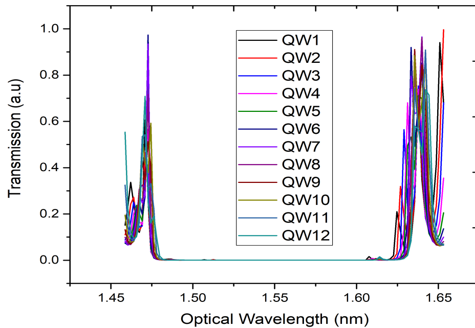
FIGURE 4.18: Transmission vs optical wavelength for 45:43 mirror ratio.
