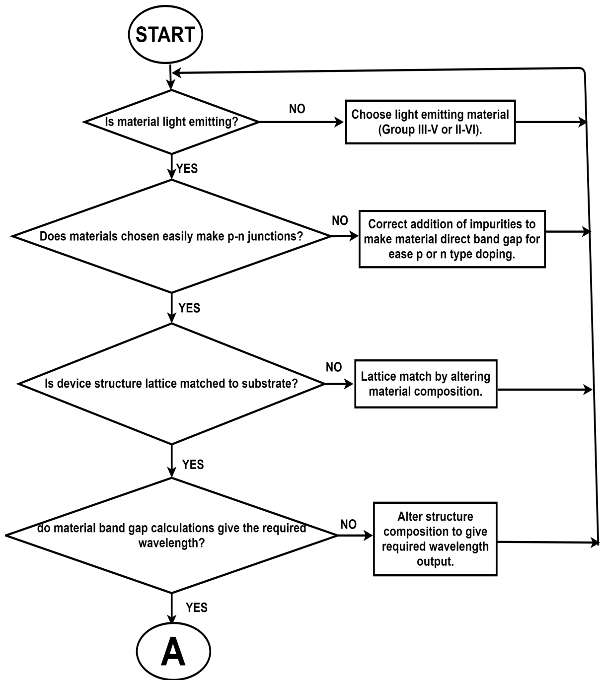
FIGURE 3.2: VCSEL development flowchart.
