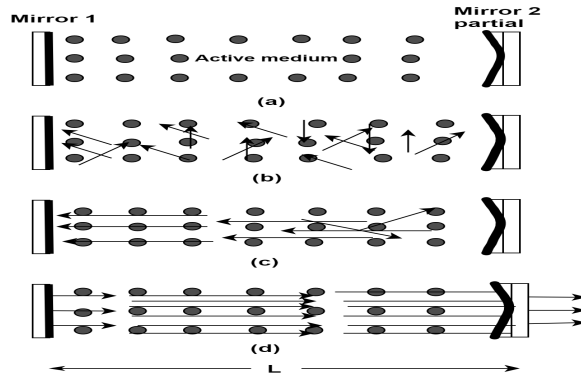
FIGURE 2.14: Cavity construction.
