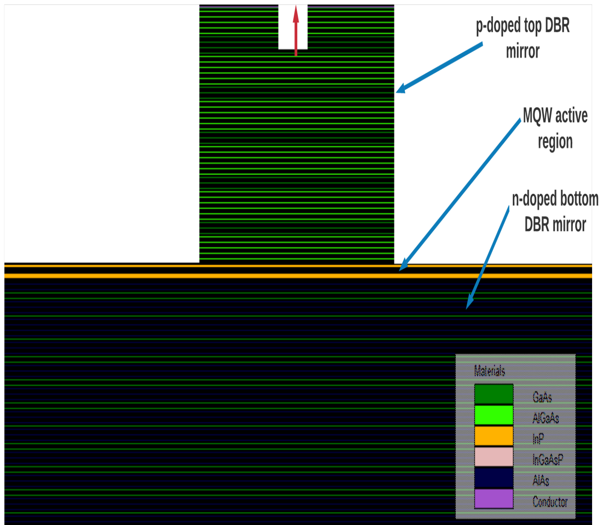
FIGURE 3.4: Simulated seven quantum well structure.
