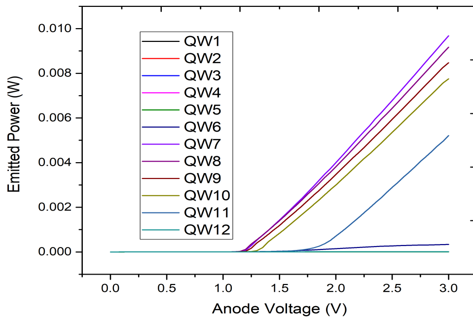
FIGURE 4.21: Emitted power vs anode voltage for 30:28 mirror ratio.
