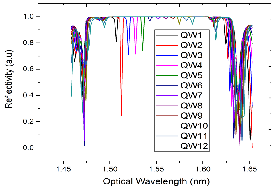
FIGURE 4.16: Reflectivity vs optical wavelength for 45:43 mirror ratio.
