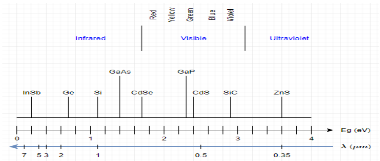
FIGURE 2.22: Band Gaps of some semiconductors.
