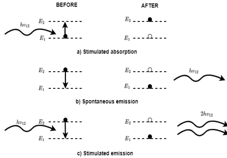
FIGURE 2.12: Illustrations on conditions for laser operation.
