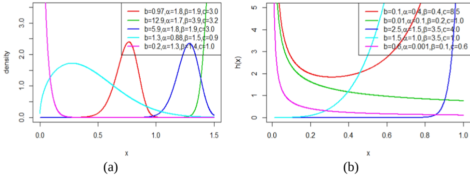
Figure 4.1: Plots of the pdf and hrf for the EOW-TL-LLoG Distribution
