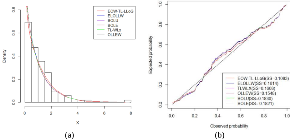
Figure 6.1: Fitted Densities and Probability Plots kevlar Data
