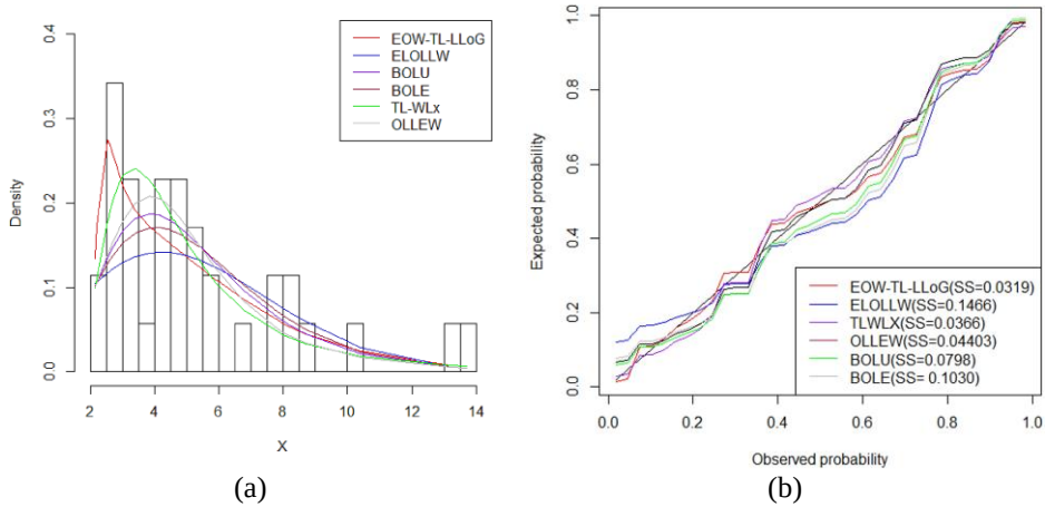
Figure 6.2: Fitted Densities and Probability Plots for Growth Hormone Data
