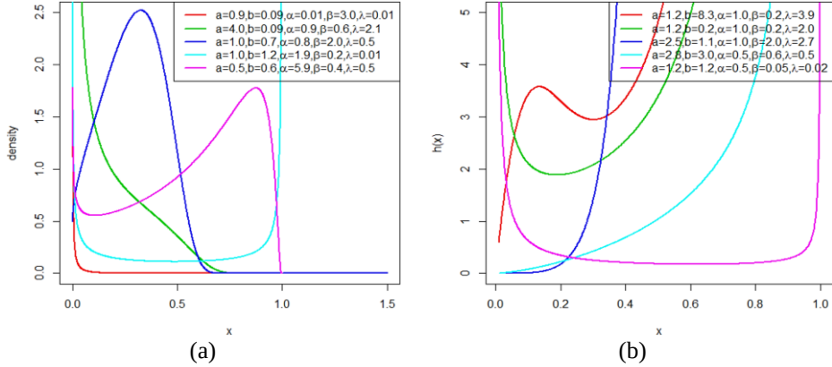
Figure 4.2: Plots of the pdf and hrf for the EOW-TL-K Distribution
