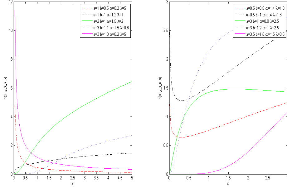
FIGURE 2. Plots of the hazard function of KPL distribution for selected values of the parameters
