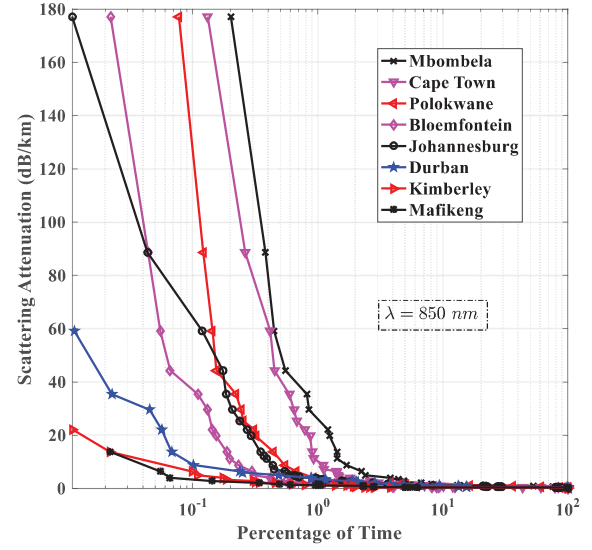
(a) 850 nm
