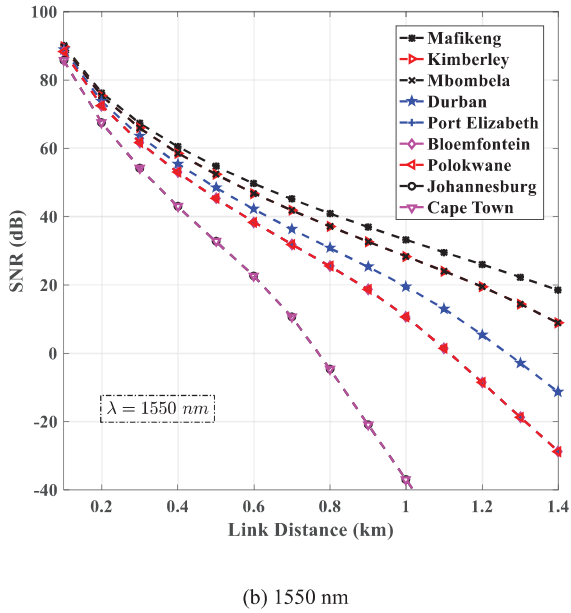
Fig. 11. Receive SNR for commercial FSO link for various cities in South Africa during foggy periods for (a) 850 nm and (b) 1550 nm.
