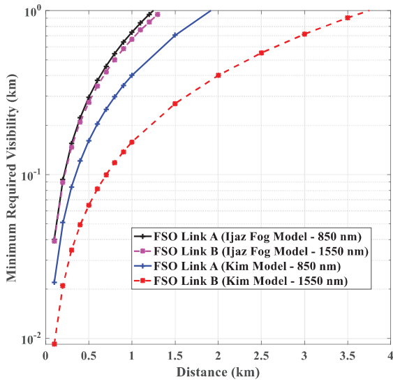
Fig. 6. Minimum required visibility vs link distance based on Ijaz and Kim models for FSO links A and B
