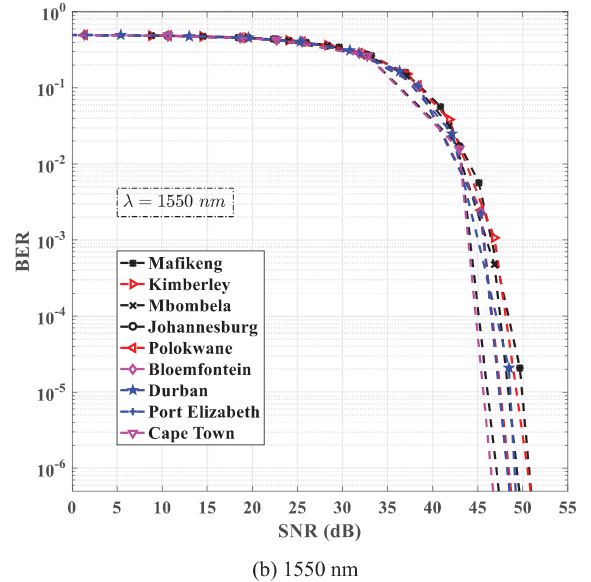
Fig. 12. BER of SISO FSO links employing OOK modulation during foggy weather and weak atmospheric turbulence for (a) 850 nm and (b) 1550 nm.
