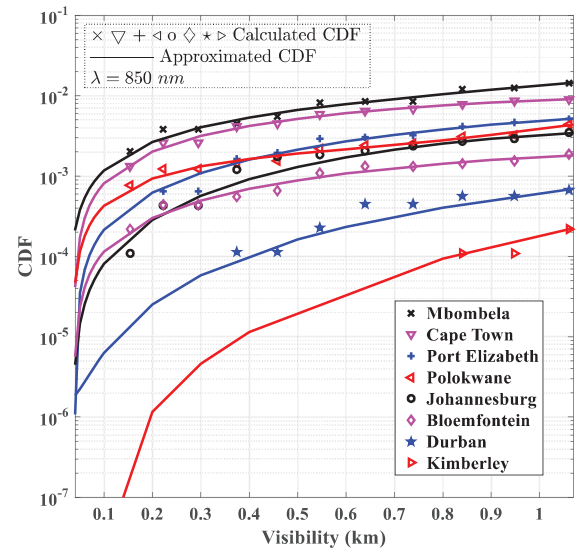
(a) 850 nm
