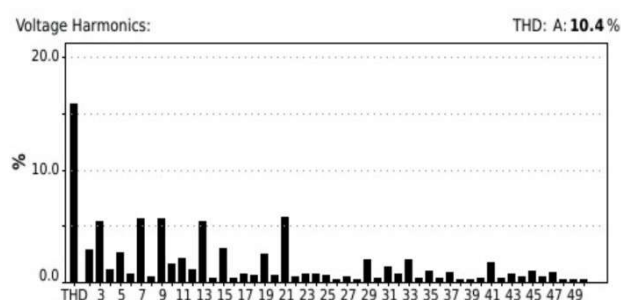
FIGURE 14. Harmonic analysis with PI controller.
