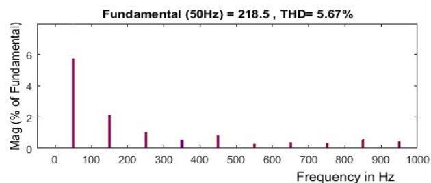
FIGURE 10. Harmonic analysis with FL controller.
