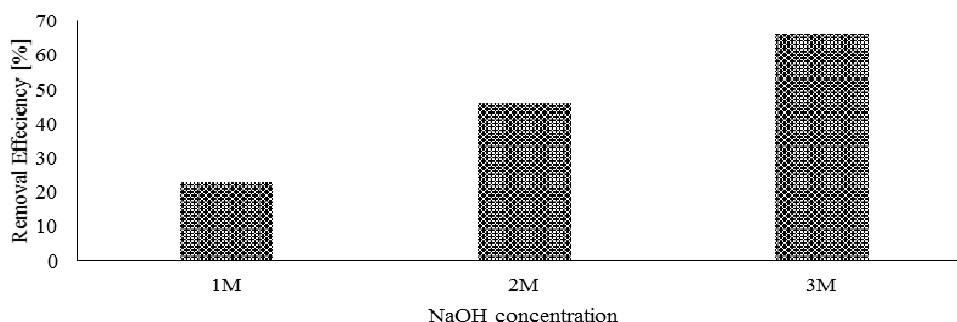
Fig. 3: CO 2 capture efficiency for absorption with NaOH
