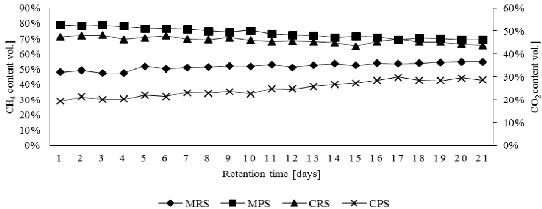
Fig. 5: Composition of biogas in absorption of CO 2 with NaOH at 2M concentration
