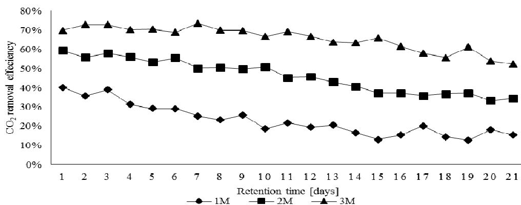
Fig. 2: Efficiency of CO_2 removal from the gas as a function of time using NaOH
