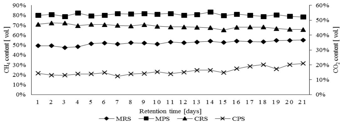
Fig. 6: composition of biogas in absorption of CO 2 with NaOH at 3M concentration
