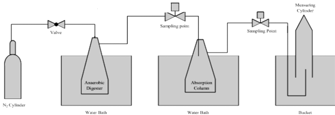
Fig. 1: Schematic diagram of lab set up for absorption of carbon dioxide using sodium hydroxide
