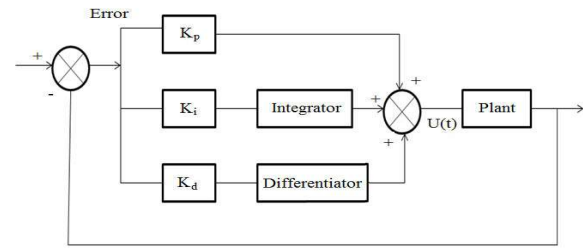
FIGURE 6. Structure of PID controller.
