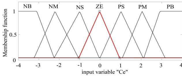
FIGURE 3. MF for the change in an error signal.
