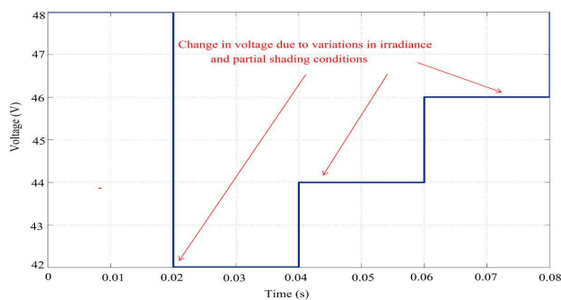
FIGURE 7. Variation of output voltage with respect to irradiance.
