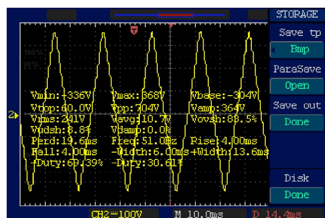
FIGURE 19. Waveform analysis for output voltage ( V_{RMS} = 241V ).
