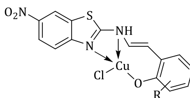
Figure 13: Antimicrobial copper complexes with hydrazone derivative ligands [67]
